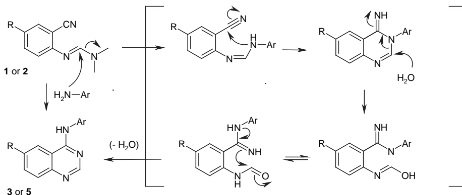
Scheme 4. Mechanism of the reaction involved in the synthesis of 4-anilinoquinazolines from anthranilonitrile.
