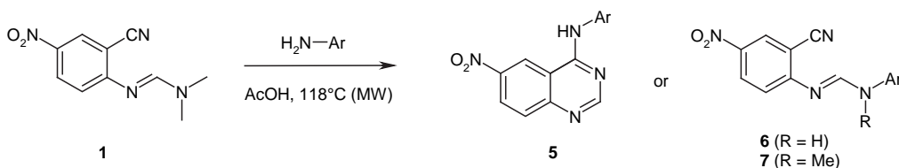
Scheme 3. Synthesis of 4-anilino-6-nitroquinazolines: for reaction times and yields see Table 1.
