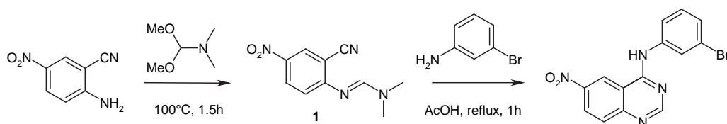
Scheme 1. Reaction described by Tsou and co-workers in 2001. 17
