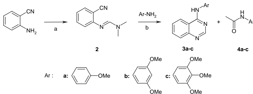
Scheme 2. Microwave-assisted synthesis of 4-anilinoquinazolines from anthranilonitriles. Reagents and conditions: (a) dimethylformamide dimethylacetal, 70 °C (800 W), 2 min, 94%; (b) acetic acid, 118 °C (600 W), 2 min, 93% ( 3a ), 94% ( 3b ) and 99% ( 3c ).
